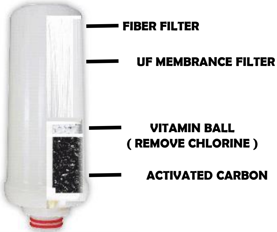
1 st FILTER UF MEMBRANCE FILTER
