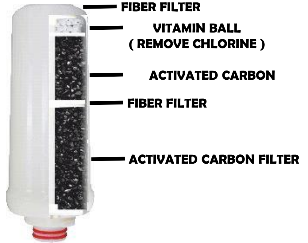
2 nd FILTER UF MEMBRANCE FILTER
